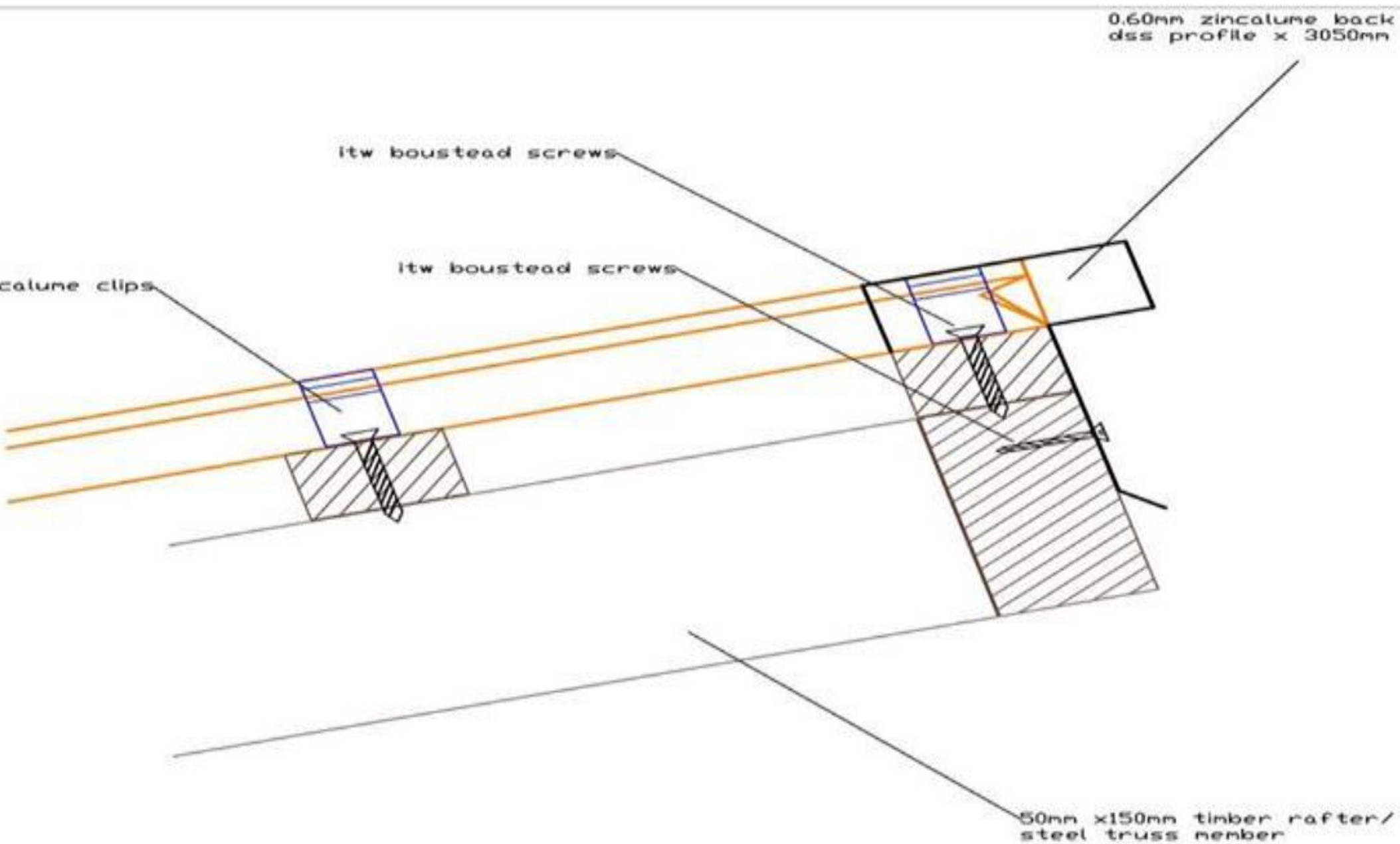
Domod standing seam (DSS) ridge detail for mono pitched roofs
