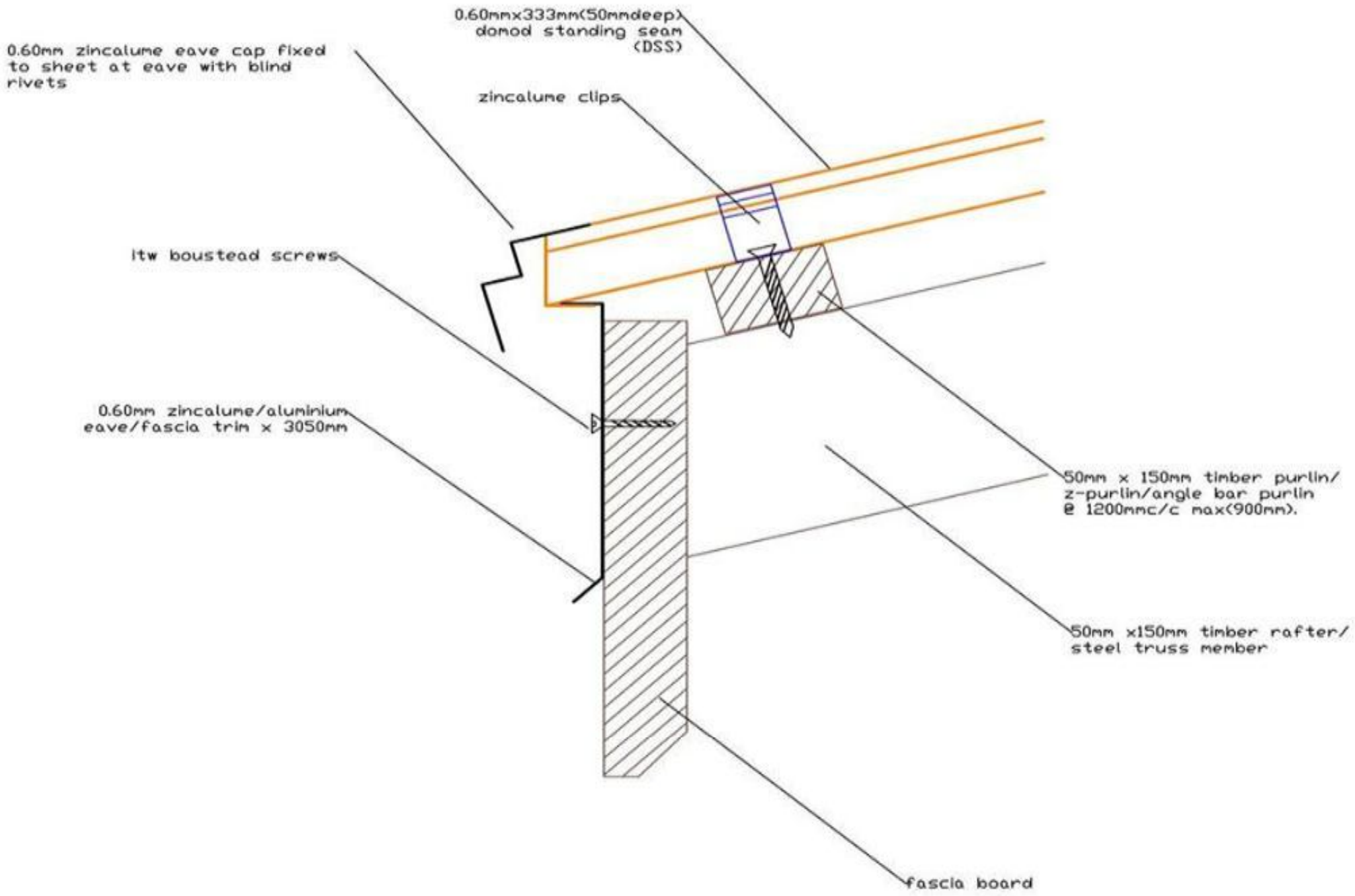
Domod standing seam(DSS) fascia detail
